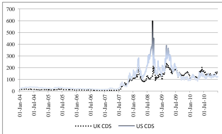
Figure 1: Basic Plot of CDS Indexes
