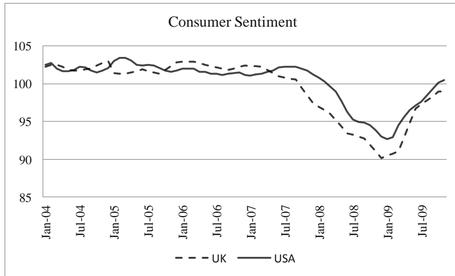
Figure 2: Consumer Sentiment (January 2004 – December 2009)
