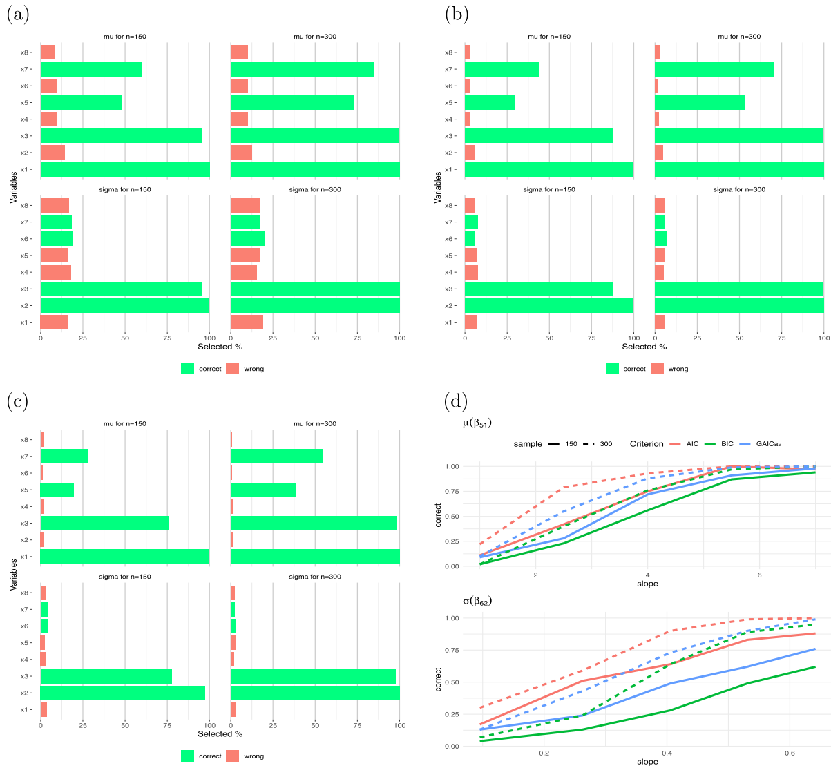
Figure 1: Selection of explanatory variables in the parametric normal heteroscedastic model. The correct/incorrect specification percentages, for different sample size, using (a) \kappa = 2 (AIC), (b) \kappa = [2 + \log(n)]/2 (GAICav) and (c) \kappa = \log(n) (BIC) criteria, and (d) different values for slope.
