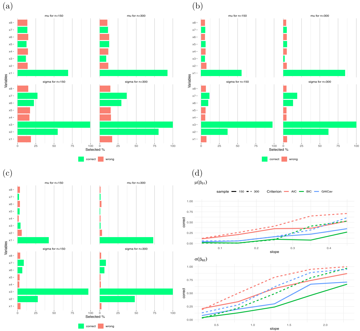
Figure 2: Selection of explanatory variables in the parametric ZIP model. The correct/incorrect specification percentages, for different sample size, using (a) \kappa = 2 (AIC), (b) \kappa = [2 + \log(n)]/2 (GAICav) and (c) \kappa = \log(n) (BIC) criteria, and (d) different values for slope.
