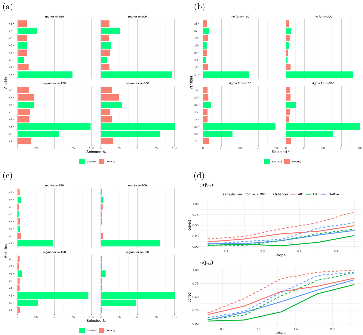
Figure 5: Selection of explanatory variables in the semiparametric ZIP model, for different sample size, using (a) \kappa = 2 (AIC), (b) \kappa = [2 + \log(n)]/2 (GAICav) and (c) \kappa = \log(n) (BIC) criteria, and (d) different values for slope.
