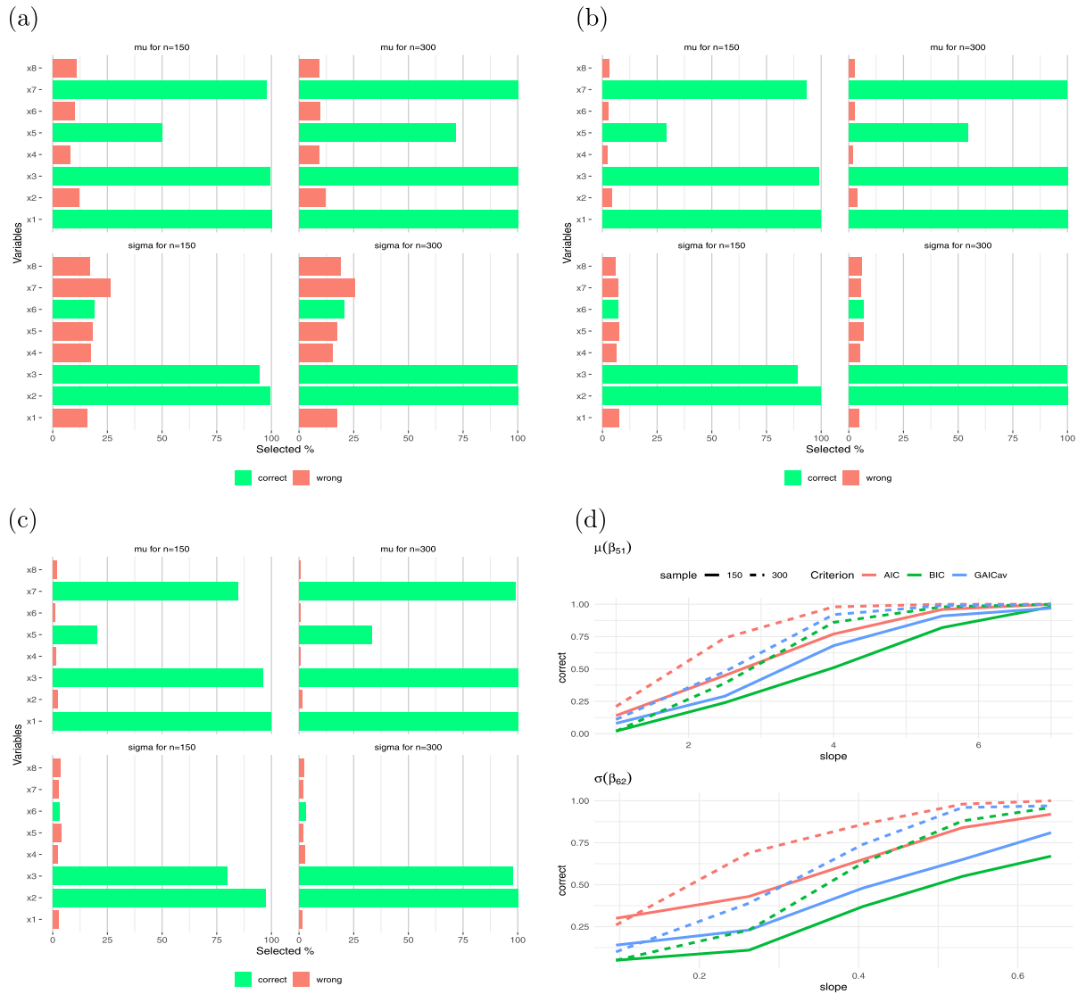
Figure 4: Selection of explanatory variables in the semiparametric normal heteroscedastic model. The correct/incorrect specification percentages, for different sample size, using (a) \kappa = 2 (AIC), (b) \kappa = [2 + \log(n)]/2 (GAICav) and (c) \kappa = \log(n) (BIC) criteria, and (d) different values for slope.
