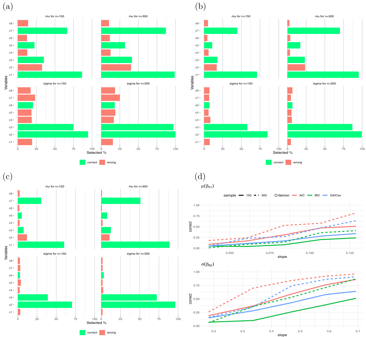
Figure 6: Selection of explanatory variables in the semiparametric Weibull model, for different sample size, using (a) k = 2 (AIC), (b) k = [2 + \log(n)]/2 (GAICav) and (c) k = \log(n) (BIC) criteria, and (d) different values for slope.
