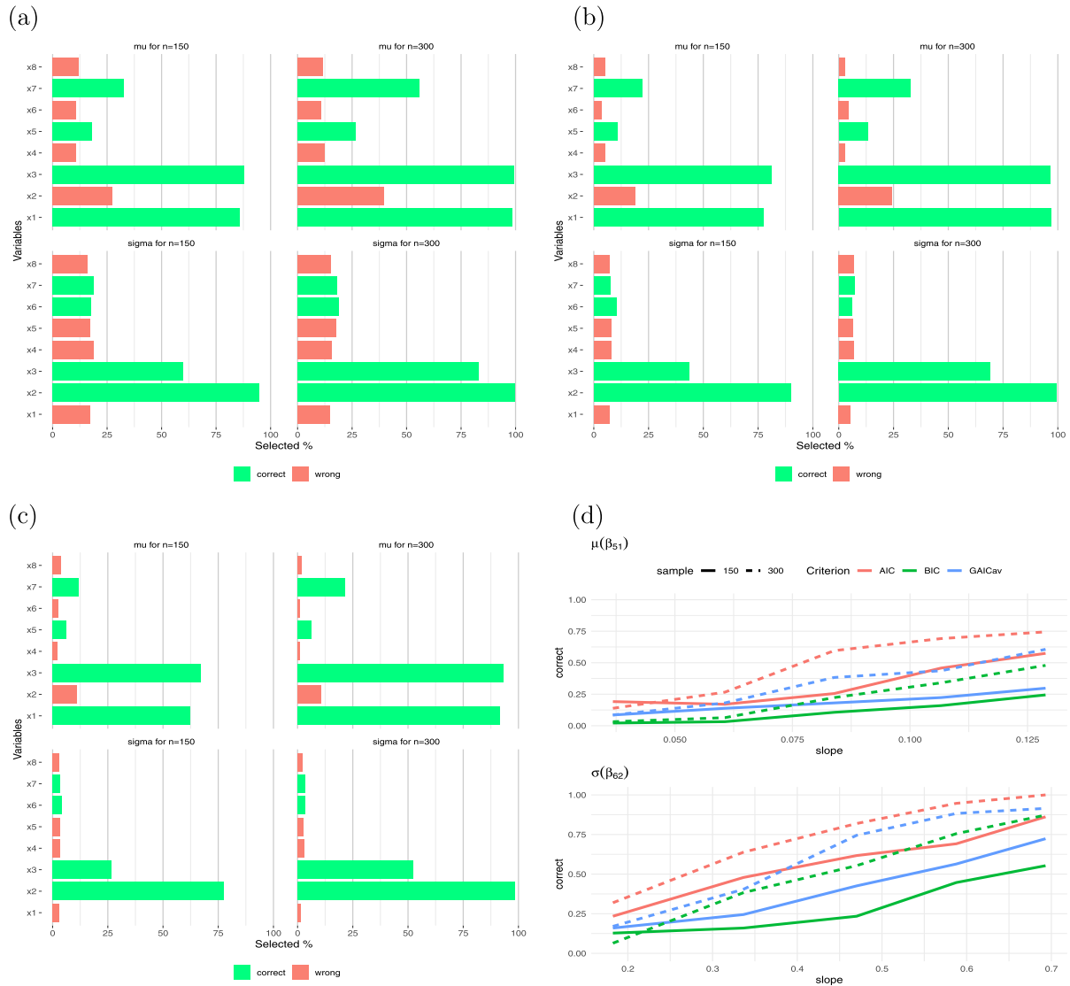
Figure 3: Selection of explanatory variables in the parametric Weibull model, for different sample size, using (a) \kappa = 2 (AIC), (b) \kappa = [2 + \log(n)]/2 (GAICav) and (c) \kappa = \log(n) (BIC) criteria, and (d) different values for slope.
